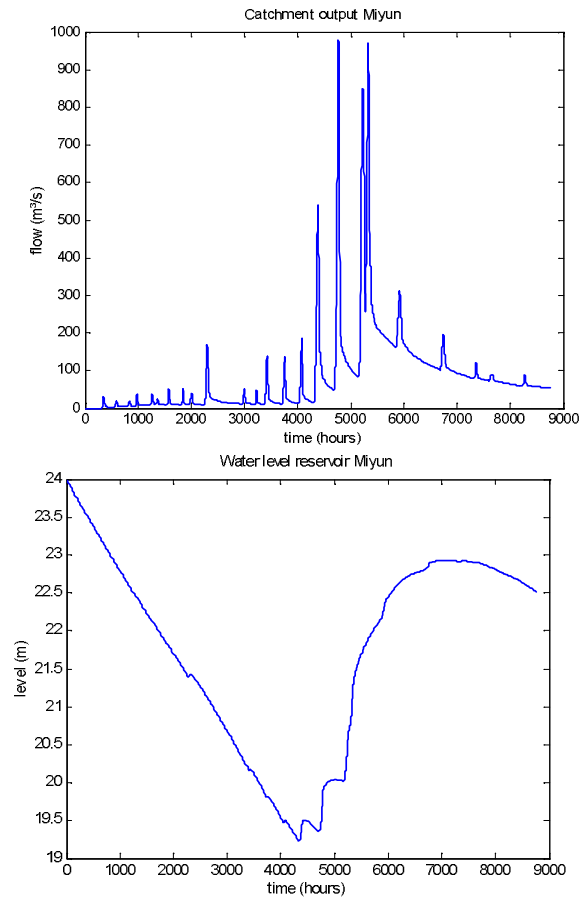
Fig. 5 Runoff from the catchment to Miyun reservoir and water level in the Miyun reservoir
