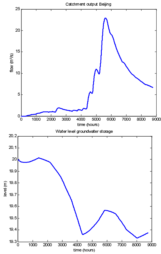
Fig. 4 Inflow of the city catchment area into the groundwater storage of the city region and the water level of this groundwater storage
